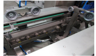
Box is clamped at three sides
