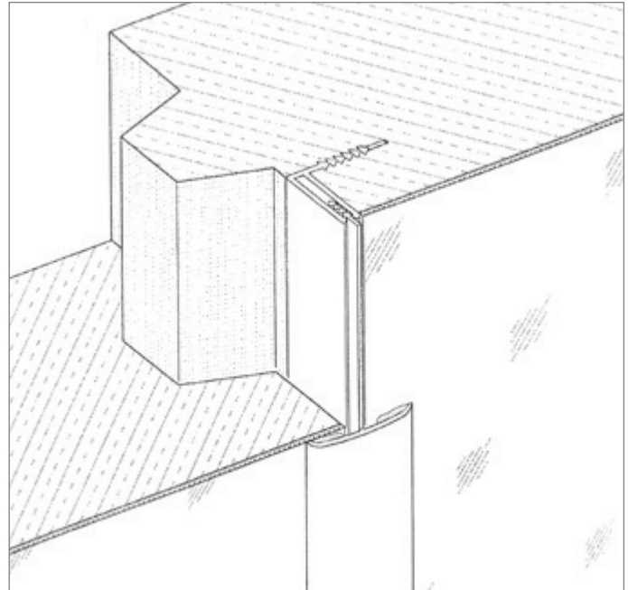
TONGUE/GROOVE PANEL WITH INSET PROFILE - CONNECTION
